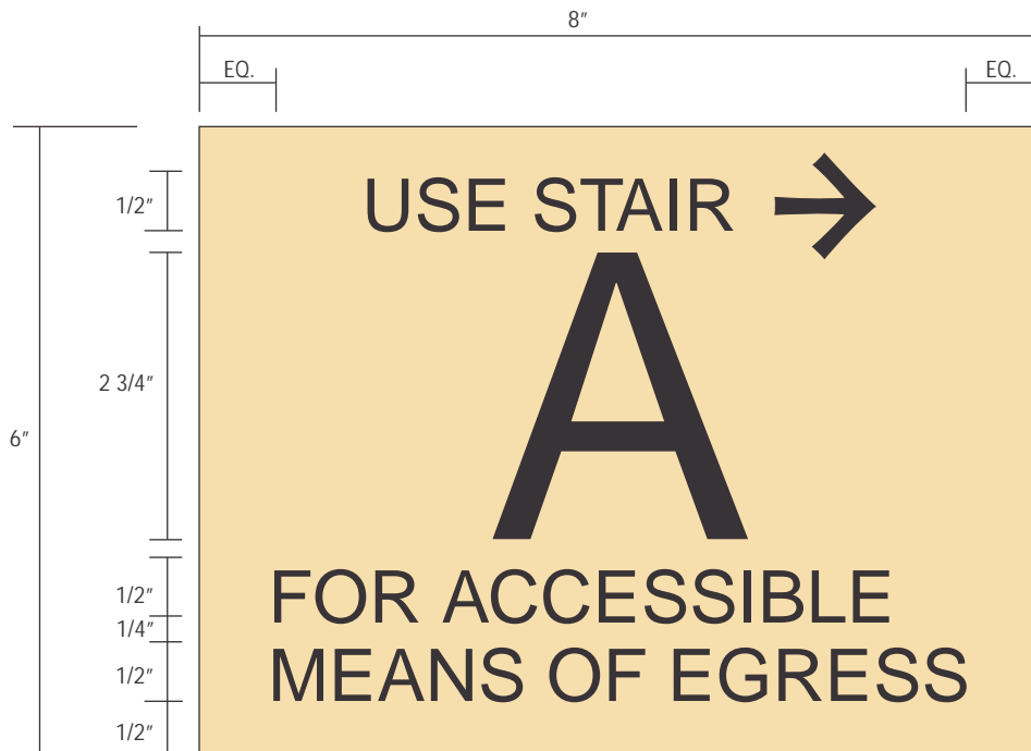
Area of Refuge Scale: 1/2" = 1"
