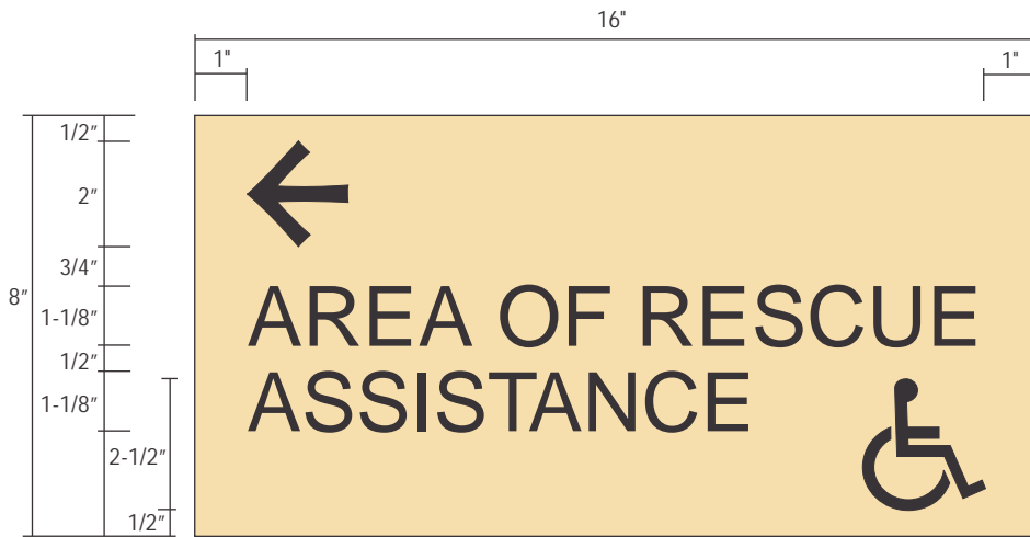
Wayfinding to Area of Rescue Assistance Scale: 1/4" = 1"
