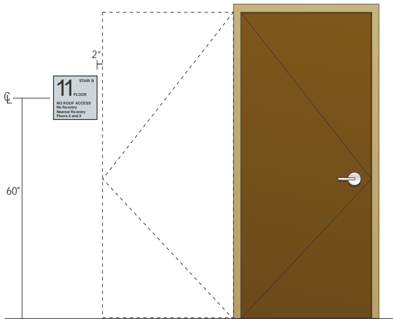
NYC Code: STAIRWELL SIDE Sign on wall to appear "free" from the door
