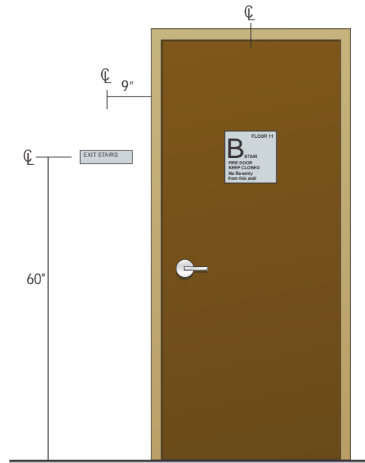
NYC Code: OCCUPANCY SIDE Sign on door and ADA/CABO component on wall
