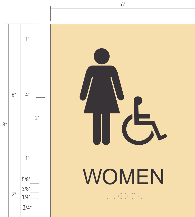
Handicapped Accessible Restroom Sign shown
