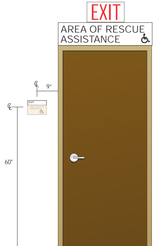
Mounting Detail: 1/2" = 1'-0"
