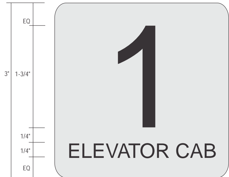
Elevator Cab Identification Plaque The mounting location must be approved by the local fire marshal.
