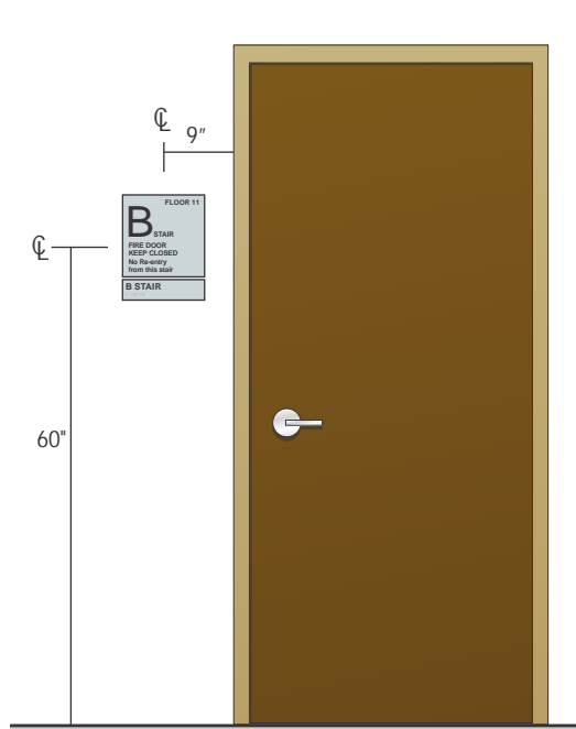
NYC Code: OCCUPANCY SIDE Sign and ADA/CABO component on wall
